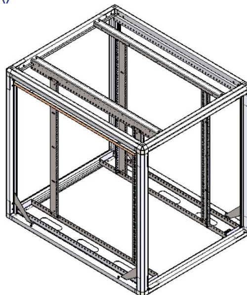
800w x 1200d Frame Assembly
