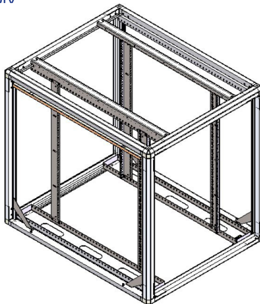
800w x 1000d Frame Assembly
