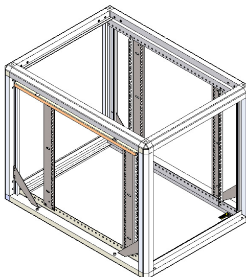
600w x 800d Frame Assembly
