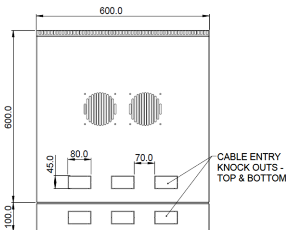
TOP VIEW - 600 DEEP WR CABINET WITH REAR HINGE BOX SECTION
