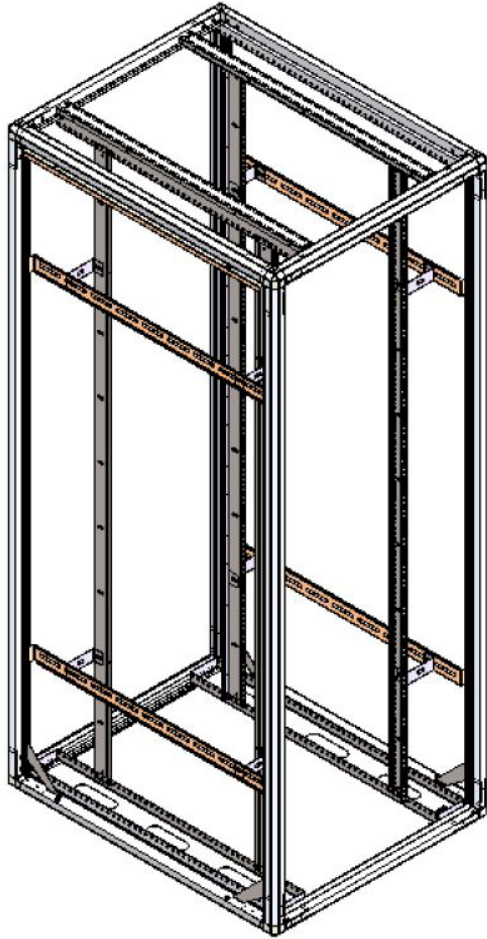
800W Cabinet Frame Assembly
